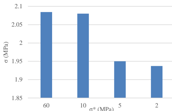
Fig. 19a Effect of interface strength on ultimate fracture stress in two-wire sample
