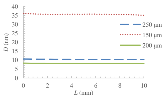
Fig. 14b Crack opening distance after activating the memory effect with different wire radius
