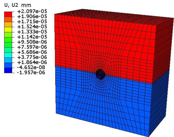
Fig. 11d Axial displacement contour for a model with 1 wire and a radius of 0.5 mm after shape memory effect
