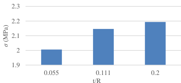
Fig. 16a The effect of capsule thickness ratio on the ultimate fracture stress in a two-wire sample
