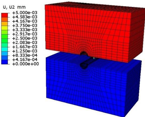
Fig. 11b Axial displacement contour for a model with 1 wire and a radius of 0.5 mm after loading
