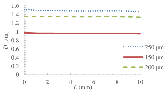
Fig. 14a Crack opening distance after loading with different wire radius
