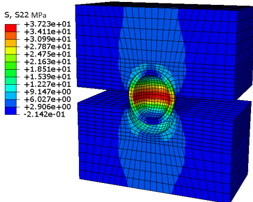
Fig. 18 Stress contour in tension direction for wireless model with 1.5 mm capsule radius
