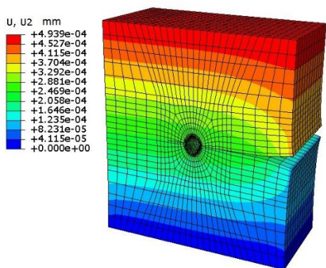
Fig. 11a Axial displacement contour for a model with 1 wire and a radius of 0.5 mm
