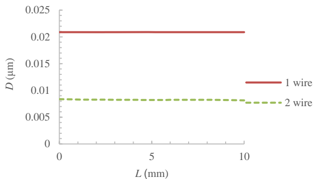
Fig. 9b Crack opening distance at the end of shape memory recovery
