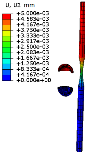
Fig. 11c Axial displacement contour of wire and a 0.5 mm capsule after loading
