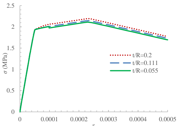
Fig. 15a The effect of capsule thickness ratio on the stress-strain diagram for a two-wire sample
