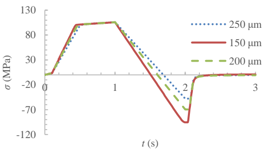
Fig. 13b Stress in the direction of applying tension in the wires under the effect of the radius of the wires
