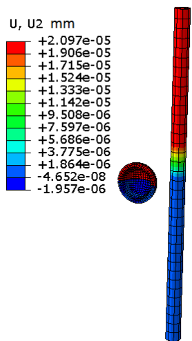
Fig. 11e Axial displacement contour of wire and a 0.5 mm capsule after shape memory effect
