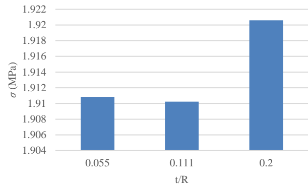
Fig. 16b Effect of capsule thickness ratio on ultimate fracture stress in wireless sample
