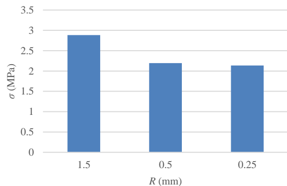
Fig. 17a The effect of microcapsule radius on the ultimate fracture stress in a two-wire sample
