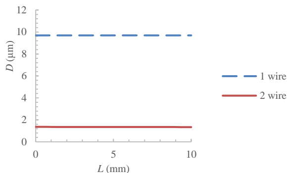
Fig. 9a Crack opening distance after unloading
