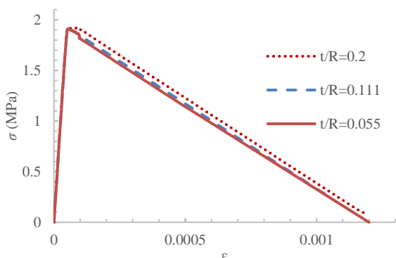
Fig. 15b The effect of capsule thickness ratio on the stress-strain diagram for a wireless sample
