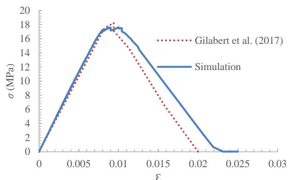
Fig. 5 Simulation results in comparison with Gilabert et al. (2017) using 2 MPa as the interface strength
