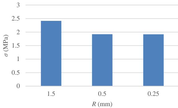
Fig. 17b Effect of microcapsule radius on ultimate fracture stress in wireless sample
