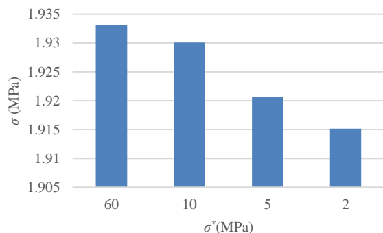
Fig. 19b Effect of interface strength on ultimate fracture stress in wireless sample
