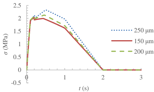
Fig. 13a Stress in the direction of applying tension in the matrix due to the radius of the wires
